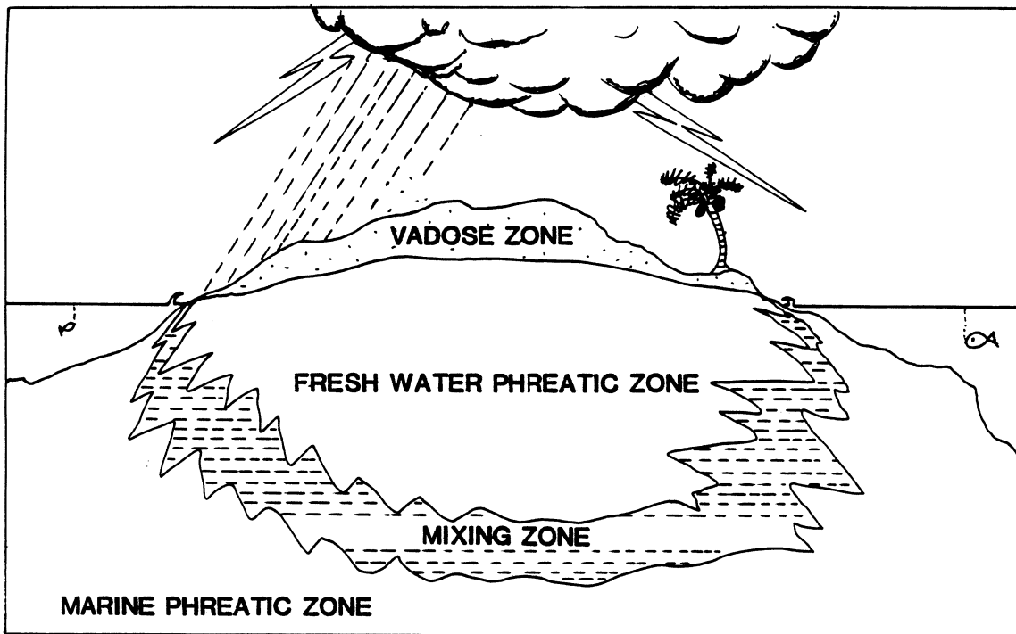
Cross-section showing the relationships between major hydrological (diagenetic) zones in an ideal, permeable carbonate island. Vertical scale, tens of metres; horizontal scale in kilometres.
